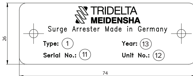
Fig. 2.2 Unit plate for multi-unit arresters
