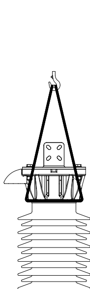
Fig. 3.1 Lifting methods
