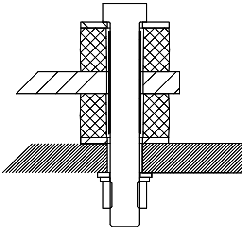
Fig. 4.1 Schematic representation of correct installation
