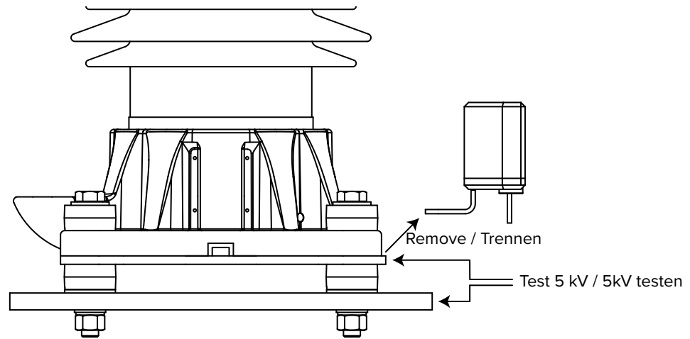
Fig. 4.2 Schematic representation of the test steps
